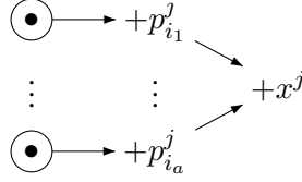
Figure 3: The net V_T^j
