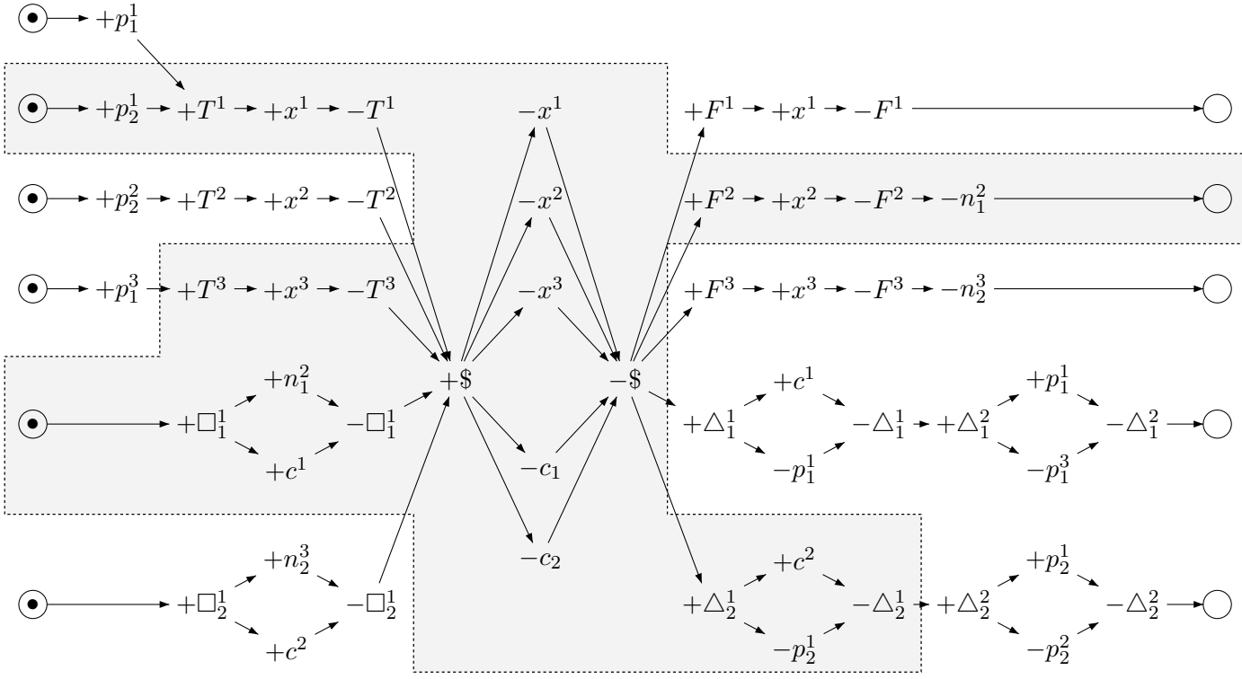
Figure 7: STG S_\varphi for \varphi \equiv (x_1 \vee \bar{x}_2 \vee x_3) \wedge (x_1 \vee x_2 \vee \bar{x}_3)
