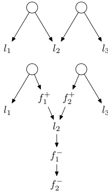
Figure 8: Transforming a 1-bounded STG into a 1-bounded free-choice STG
