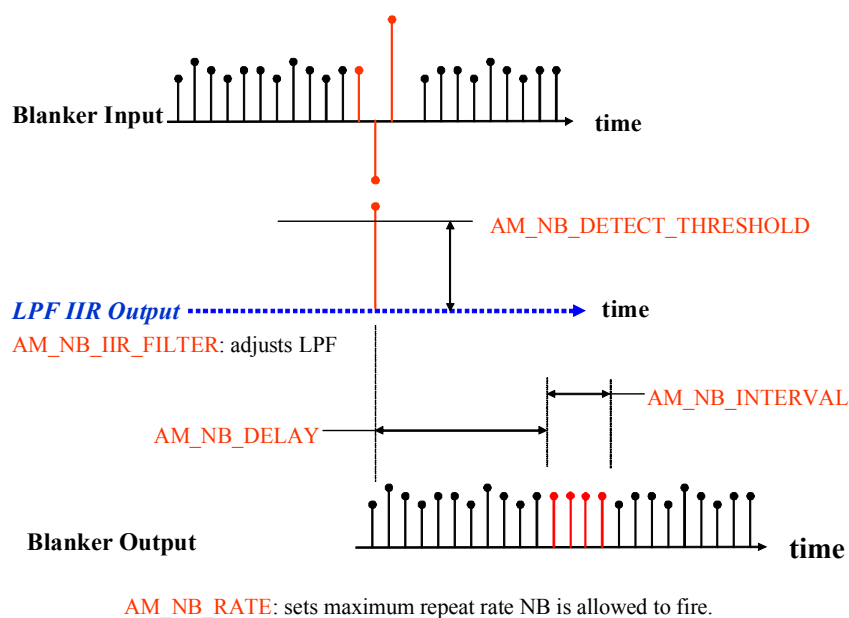
Figure 13. AM Noise Blanker
