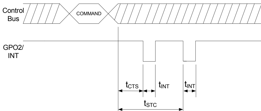
Figure 29. CTS and STC Timing Model
