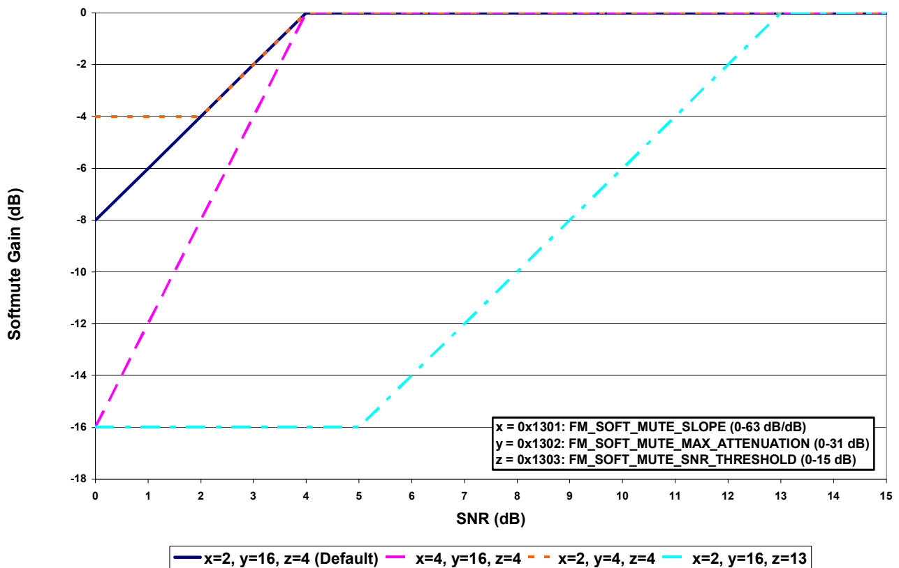
Figure 3. Softmute Gain (dB)
