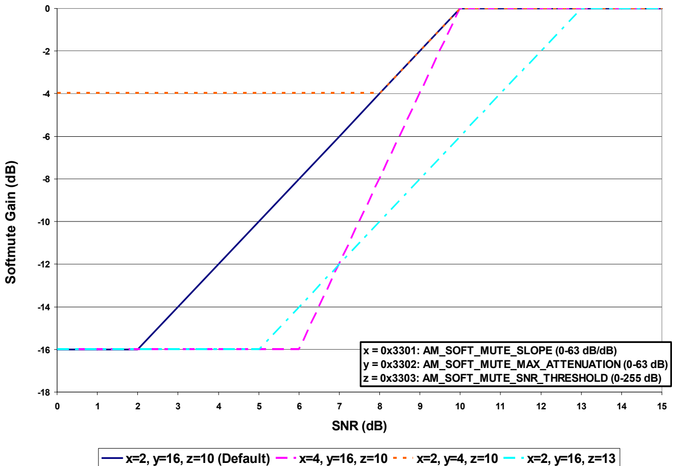
Figure 14. AM Softmute SNR
