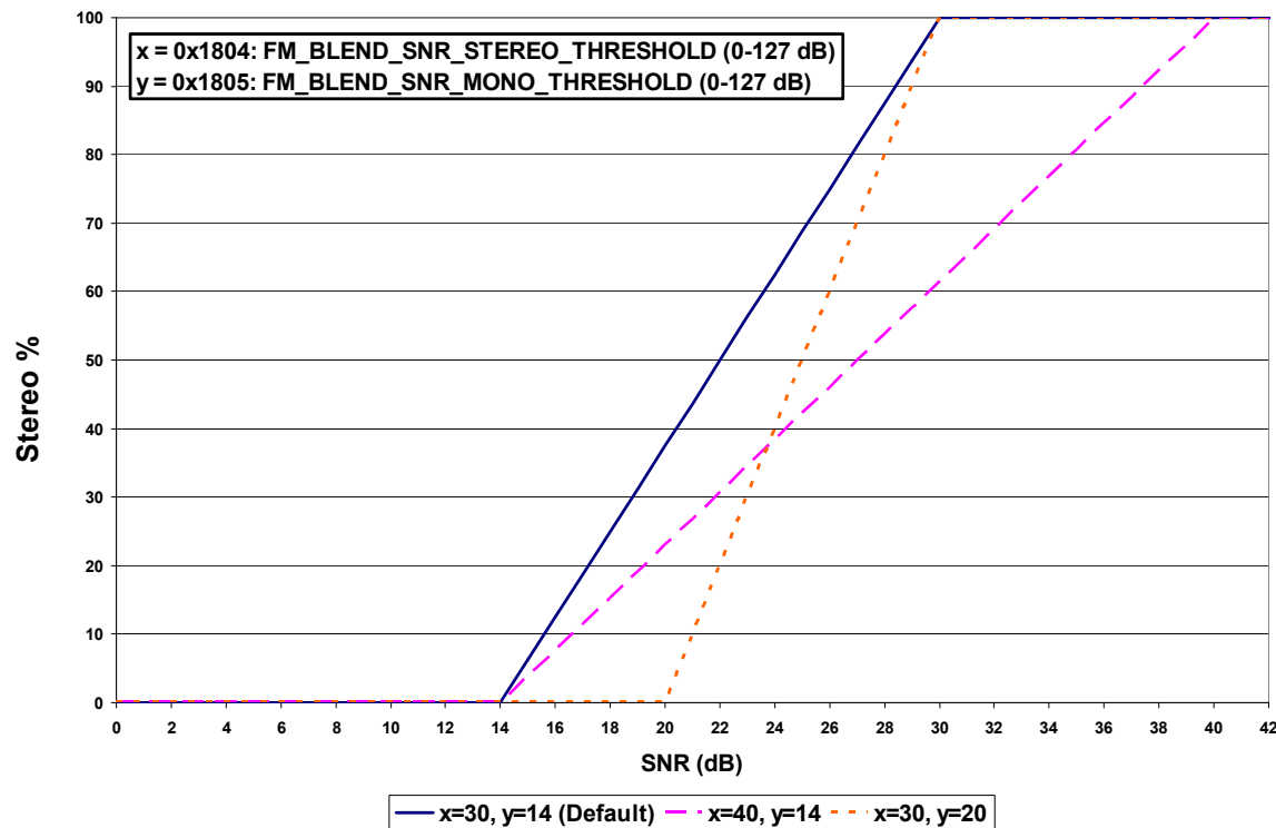
Figure 5. SNR Blend
