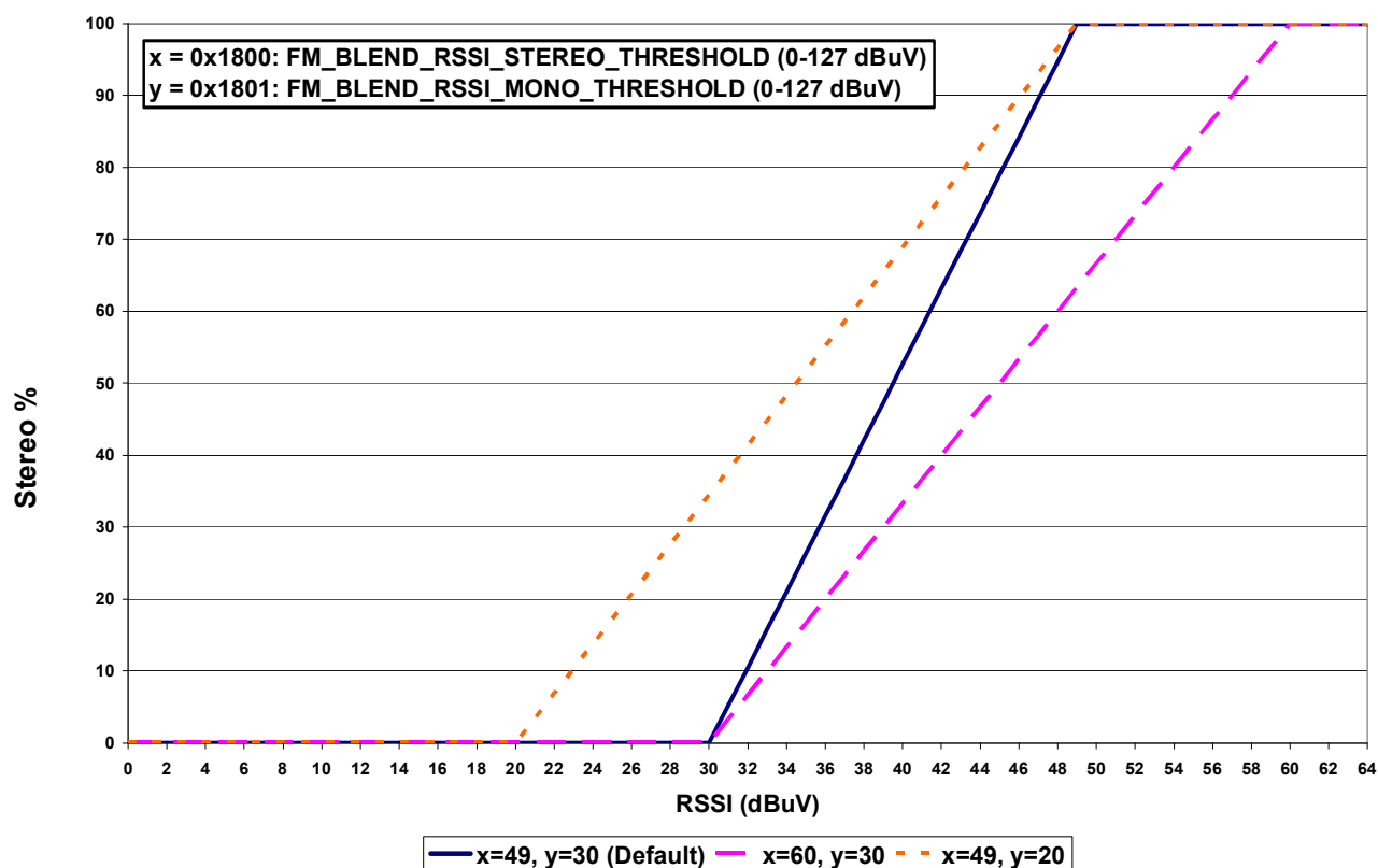
Figure 4. RSSI Blend
